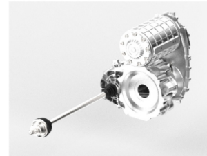
Gearbox_and_AC_Motor
